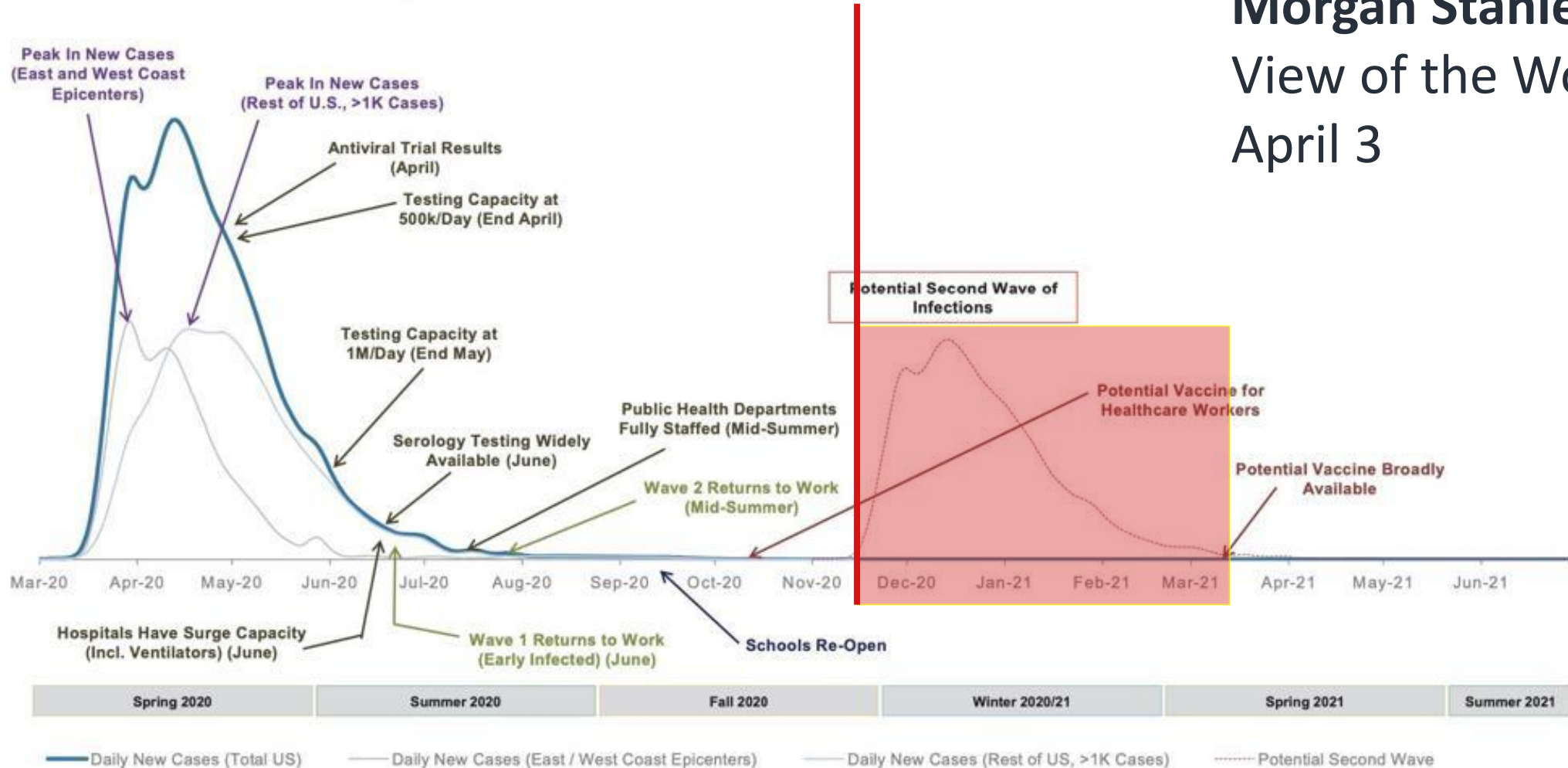
Actual/Estimated New Case Count (United States, Non-Cumulative)
